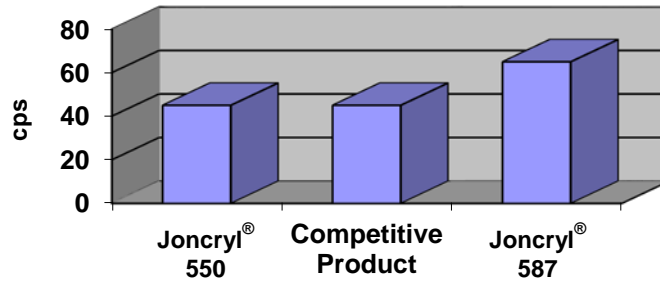
Viscosity of Automotive Refinish Clears at 4.8 lbs/gal VOC
